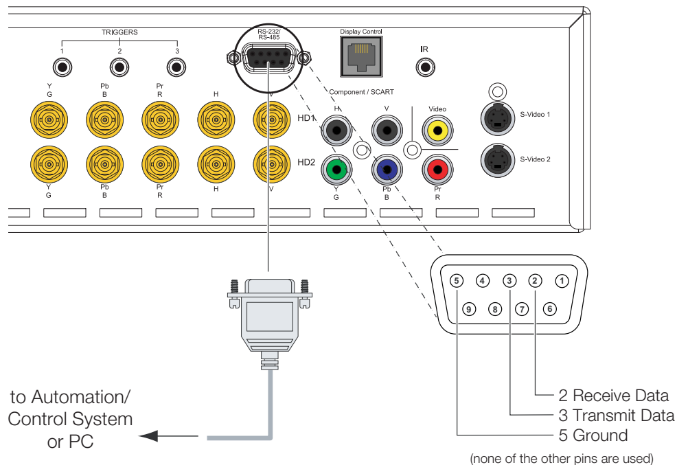
Figure 3-16. RS-232 Control System Connection
