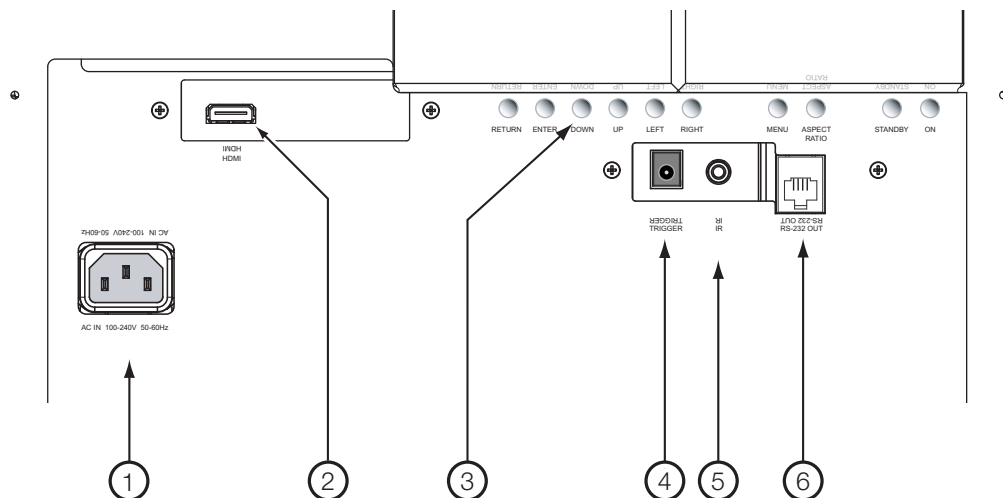
Figure 2-2. VX-6000d Rear Panel
